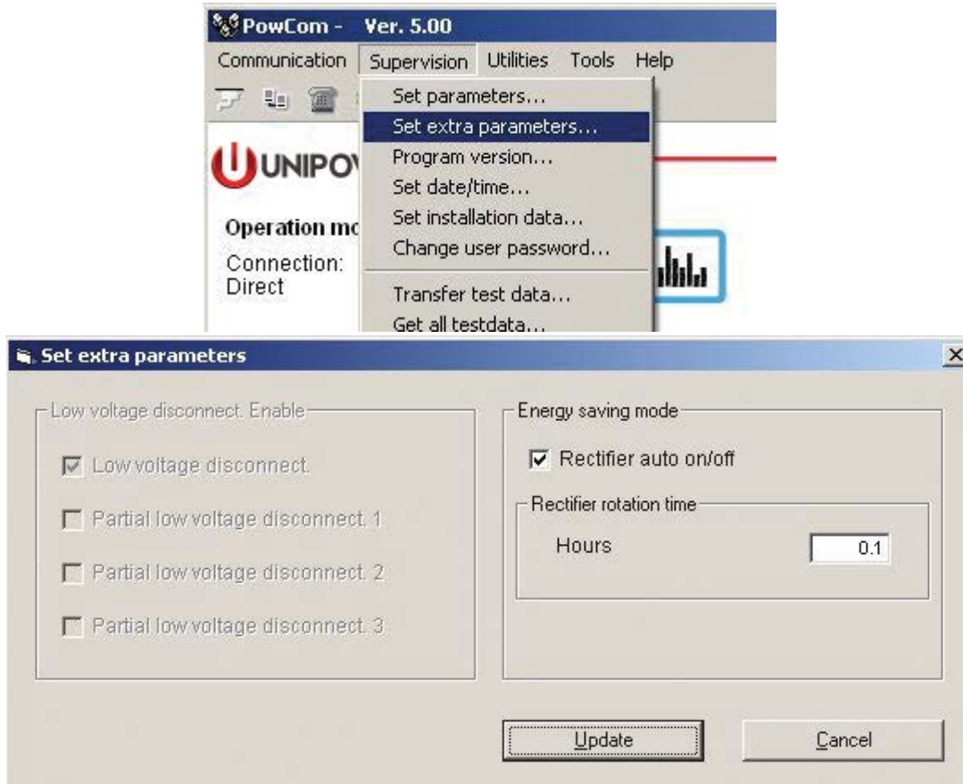
Figure 4 - PowCom™ menu steps
