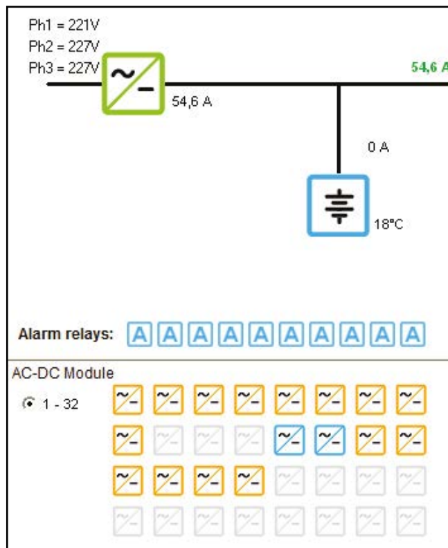
Figure 5 - PowCom™ window: Energy Saving in operation
