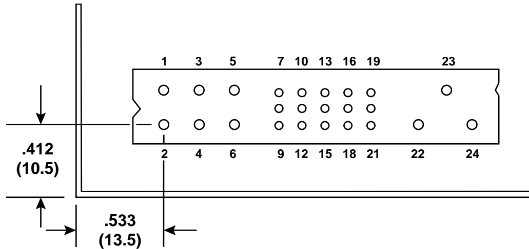
Figure 4 – Module connection details
