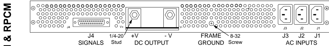
Figure 7a – Model TPCM1U3 with IEC60320- C14 Connectors
