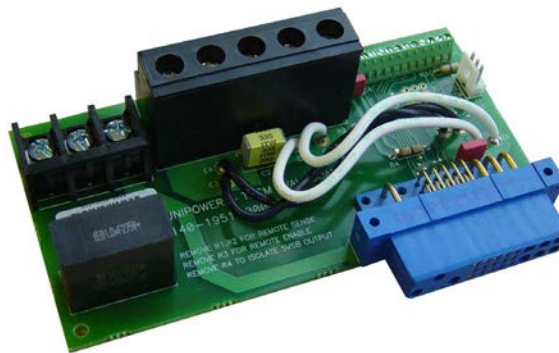
Figure 5 – Radian Mating Interface Board
