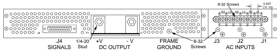
Figure 7c – Model TPCPR1U3A with Terminal Block Connections
