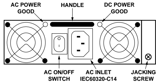
Figure 2b - Front Panel View TPCMxxxx-E
