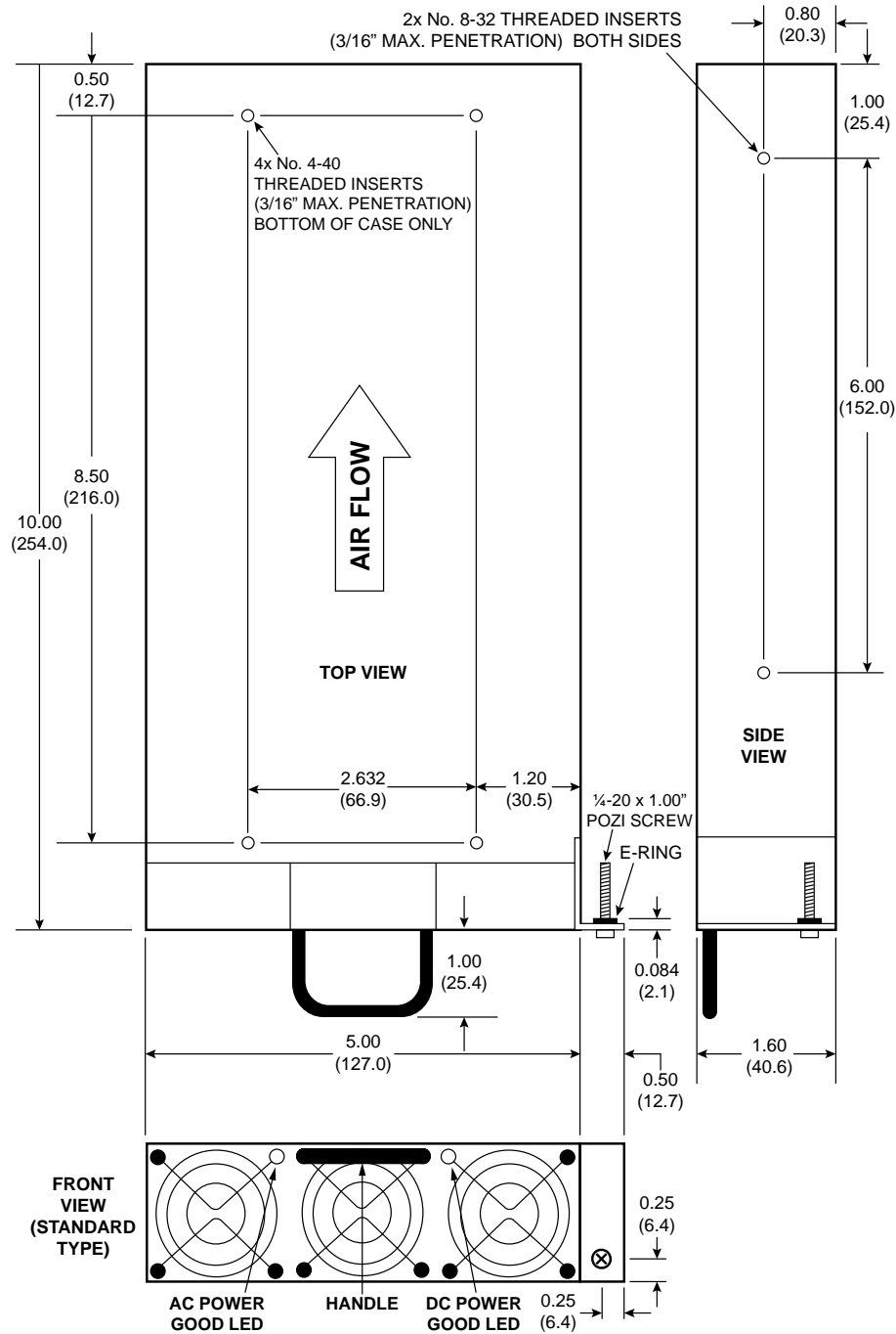
Figure 3 - Module Dimensions
