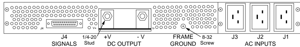
Figure 7e – Model TPCPR1U3C with IEC60320-320 C20 Filtered Connections
