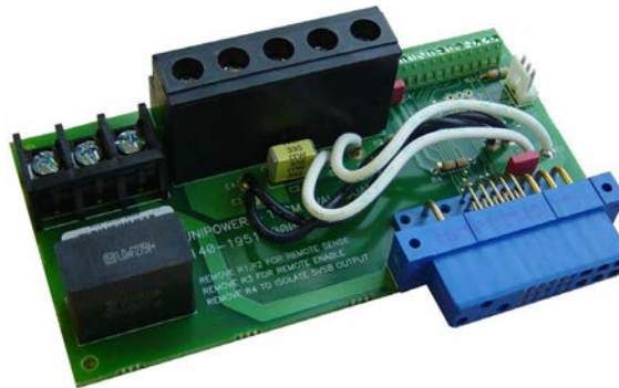
Figure 5 – Radian Mating Interface Board
