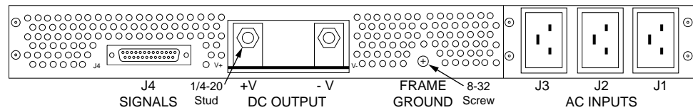
Figure 7d – Model TPCPR1U3B with IEC60320-C20 Connections
